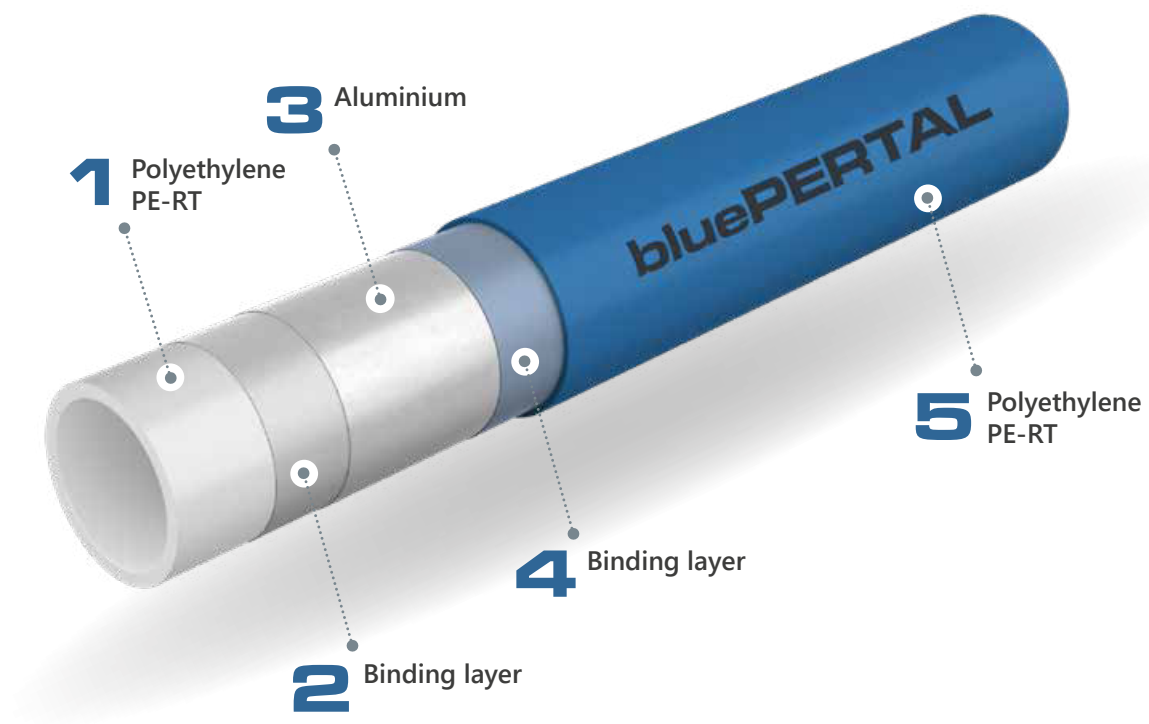
Fig. 46. Design of bluePERTAL with aluminum layer.
