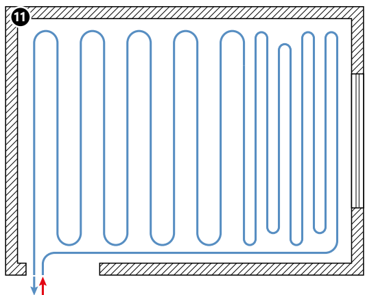
Fig. 11. Floor heating/cooling coil in the series pattern, with an edge zone made on a single loop, arranged along the external wall or surface with large glazing.
