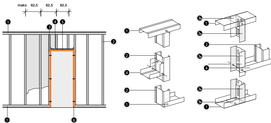
Fig. 39. The diagram of mounting the frame to the supporting construction (dimensions in cm). 1. UW profile. 2. CW profile. 3. CW or UA stiffening profile. 3a. UA stiffening profile. 3b. UA square. 4. UW latch. 5. Frame. 6. Connector.
