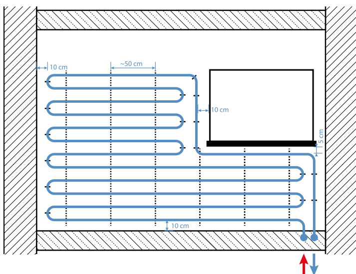
Fig. 34. Assembly distances in wall heating.
