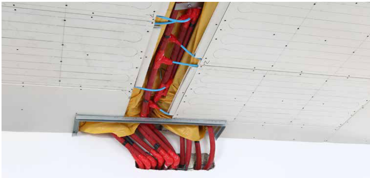
Fig. 6. Ceiling cooling installation using heating and cooling panels of KAN-therm Wall system.
