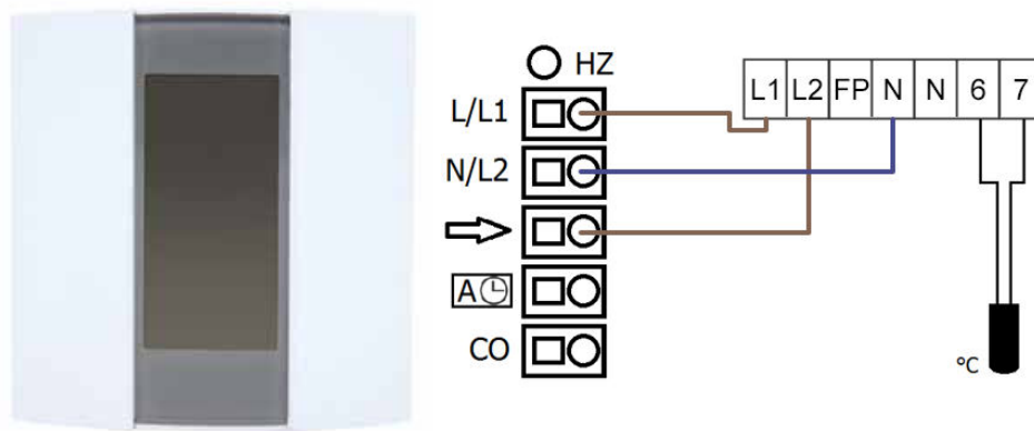
Fig. 64. Diagram of wiring of weekly regulator for heating to the Basic+ 230 V terminal block (with the option of floor temperature sensor).
