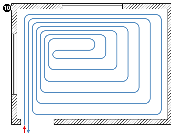
Fig. 10. Floor heating/cooling coil in the spiral pattern, with an edge zone made on a single loop, arranged along the external walls or surfaces with large glazing.
