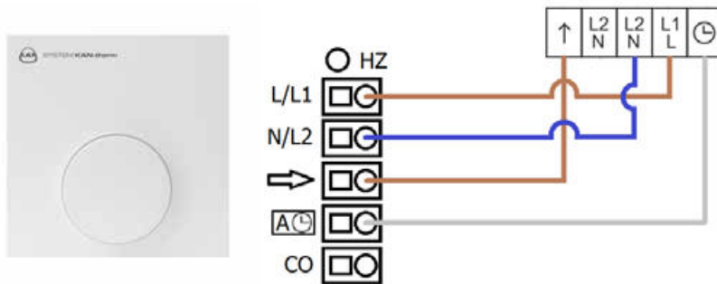
Fig. 61. Diagram of wiring of temperature sensor to the Basic+ 230 V or 24 V terminal block (with the option of periodic temperature reduction by connecting an external clock)
